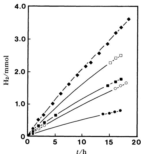
Fig. 2. Time-course plot of dihydrogen evolution from methanol with [\text{Ru}(\text{OAc})\text{Cl}(\text{PEtPh}_2)_3] catalyst. [\text{Ru}(\text{OAc})\text{Cl}(\text{PEtPh}_2)_3] : (●) 0.50 \text{ mmol dm}^{-3} , (○) 1.0 \text{ mmol dm}^{-3} , (■) 1.5 \text{ mmol dm}^{-3} , (□) 2.5 \text{ mmol dm}^{-3} , (◆) 5.0 \text{ mmol dm}^{-3} . Methanol 200 \text{ ml} , 65^\circ\text{C} (refluxing).
